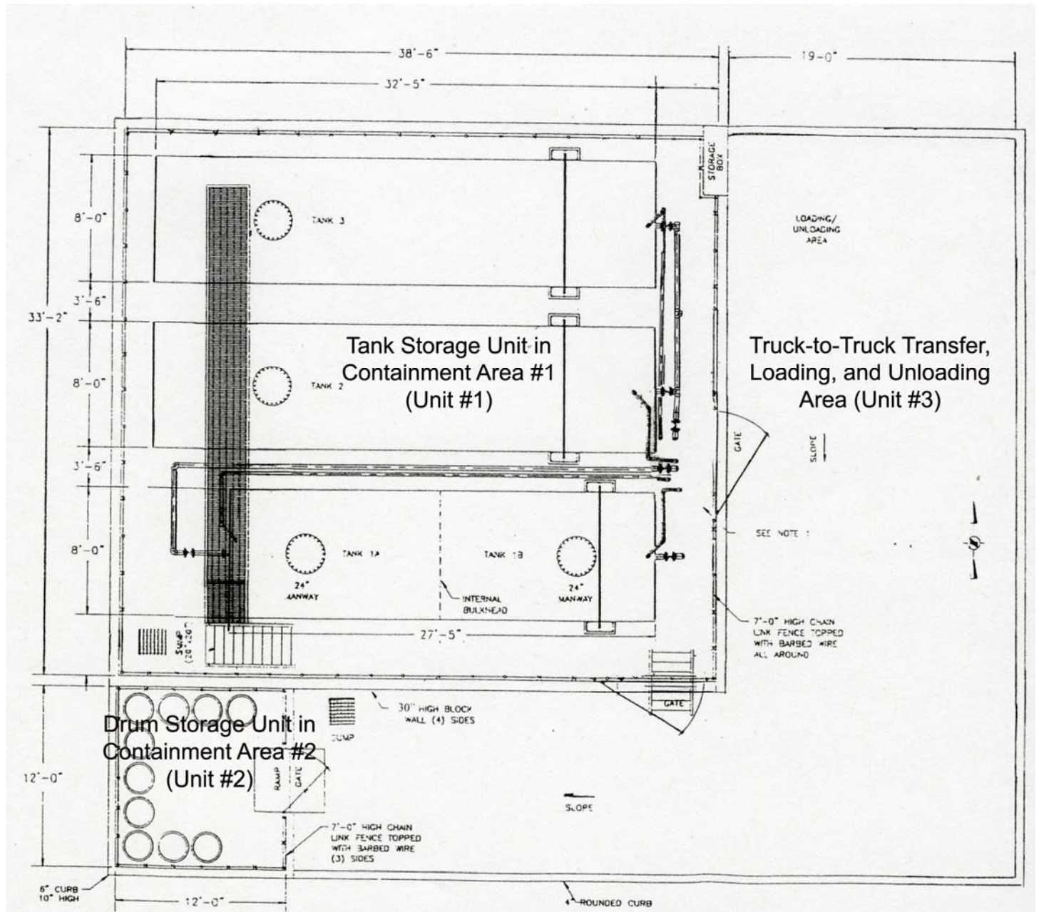
Figure 2. Facility Site Plan
