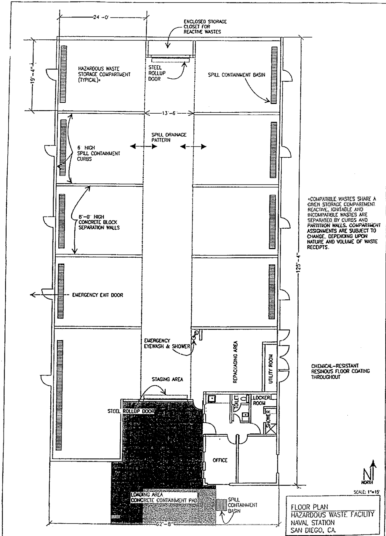
APPENDIX A - FACILITY FLOOR PLAN
